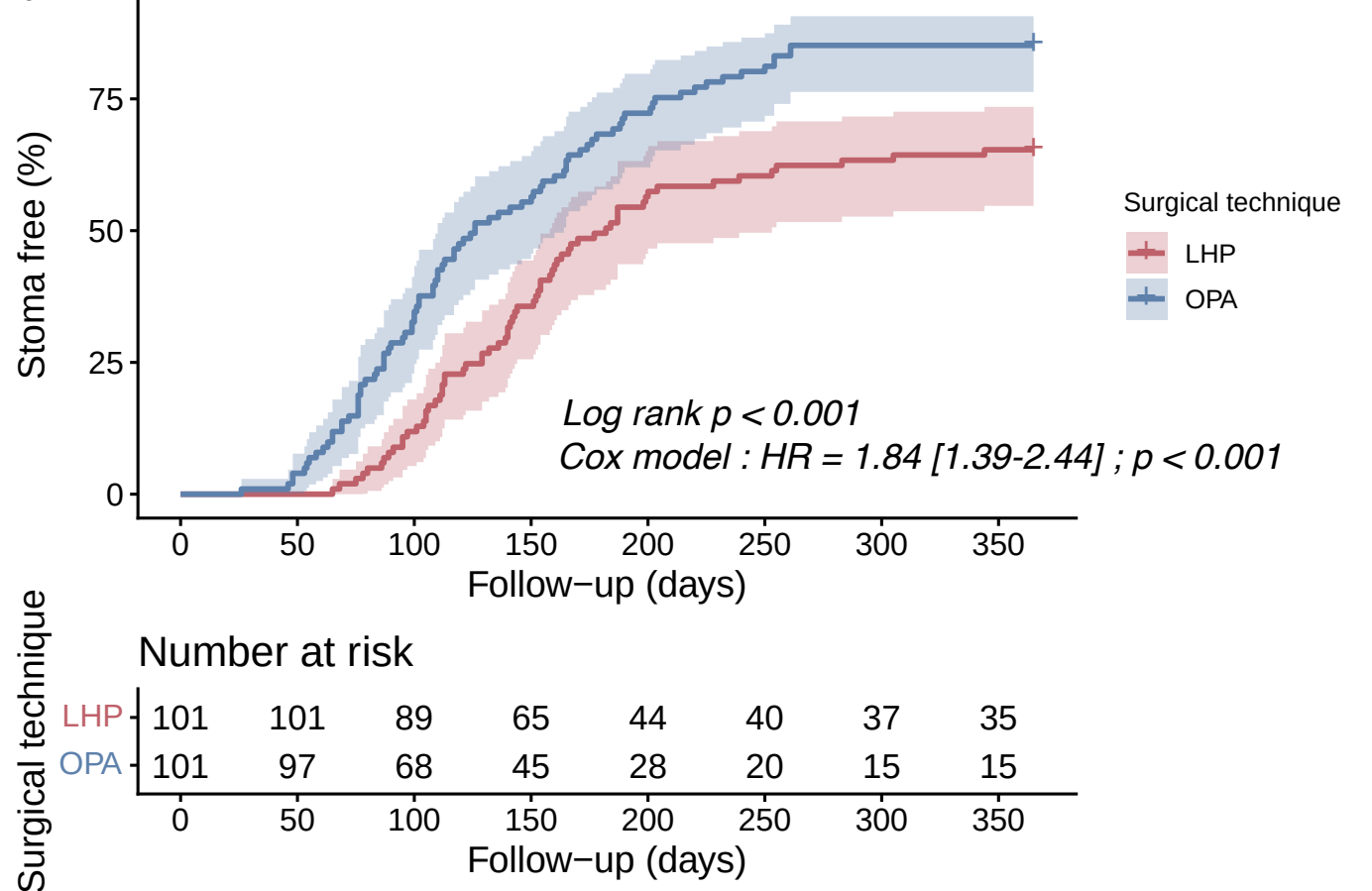
Figure 2 : Stoma-Free Survival
